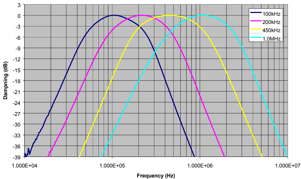
Filter Module S00011 LF-UT
